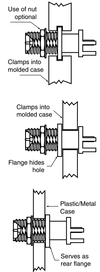
MOUNTING METHODS
